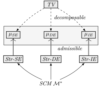
Figure 3.1: Fundamental Problem of Causal Fairness Analysis (TV version).
