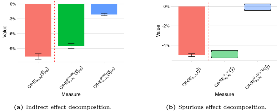
Figure 6.16: Further decomposition of the spurious and indirect effects on COMPAS.
