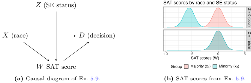
Figure 5.9: SFM and SAT scores visualization in Ex. 5.9.
