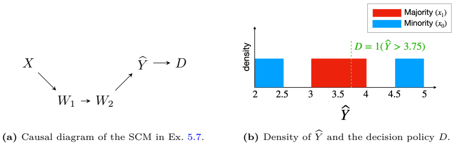
Figure 5.8: Causal diagram and the density of the GPA predictor \hat{Y} for Ex. 5.7.
