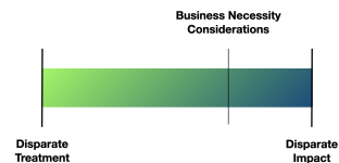
Figure 1.1: The spectrum of fairness notions spanned by the disparate treatment and disparate impact doctrines.
