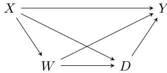
Figure 5.11: Causal diagram for Ex. 5.11 (breast cancer) and Ex. 5.13 (startup professional development courses).
