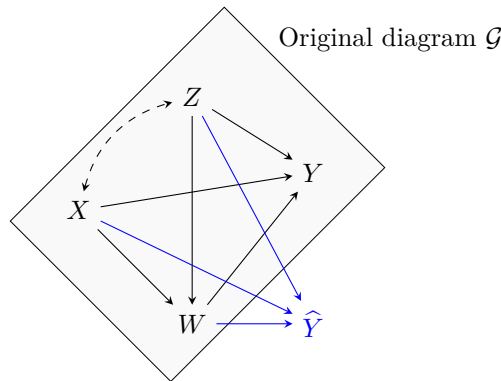
Figure 5.4: Standard Fairness Model (SFM) extended with a blue node \hat{Y} , for the task of (fair) prediction.
