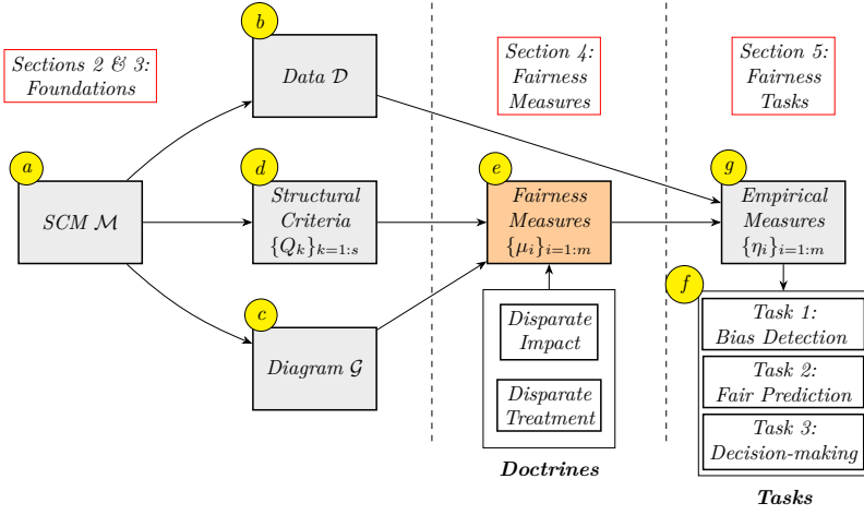
Figure 1.3: A mental map of the Causal Fairness Analysis framework.
