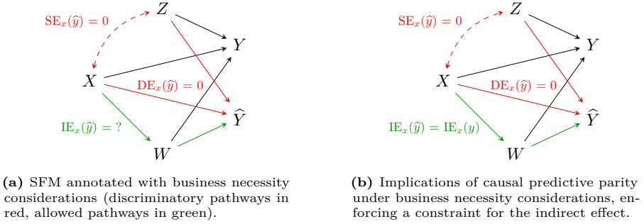
Figure 4.9: Business Necessity and Causal Predictive Parity (CPP).
