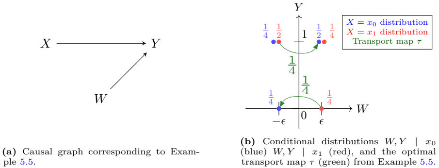
Figure 5.7: Causal diagram and distribution from Ex. 5.5.
