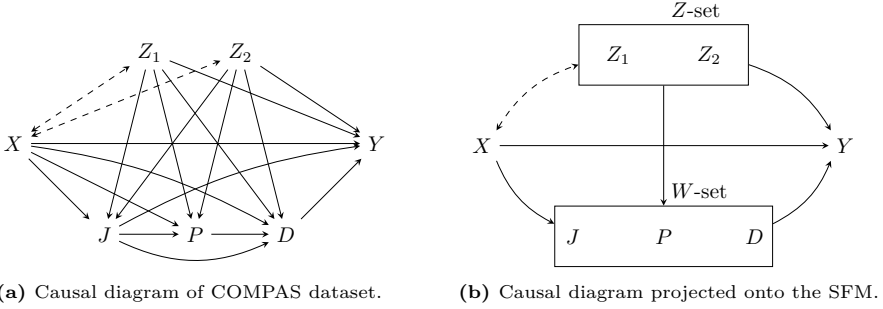
Figure 2.1: Causal diagram of COMPAS dataset and its projection onto the SFM.
