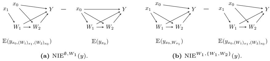
Figure 6.13: Graphical representation of how the NIE is decomposed in Ex. 6.16.
