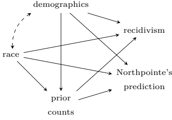
(a) SFM for Ex. 5.3.
