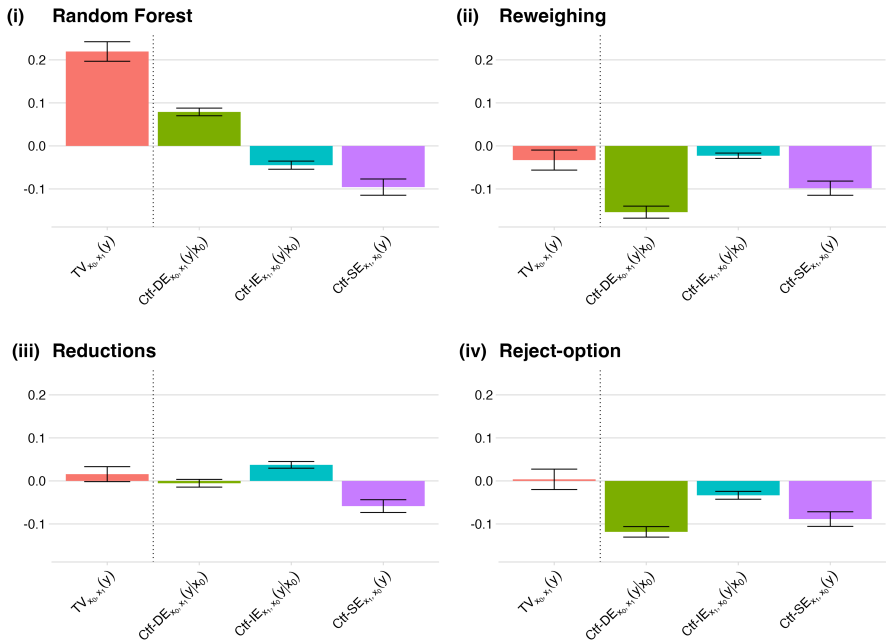
Figure 5.6: Causal Fairness Analysis applied to a standard prediction method (random forest, subfigure (i)) and three different fair prediction algorithms: reweighing (Kamiran and Calders, 2012) in subfigure (ii), reductions (Agarwal et al. , 2018) in subfigure (iii), and reject-option (Kamiran et al. , 2012) in subfigure (iv). All of the fair predictions methods reduce the TV measure, but fail to nullify the causal measures of fairness. Confidence intervals of the measures, obtained using bootstrap, are shown as vertical bars.
