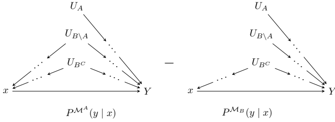
Figure 6.8: Quantity \text{Exp-SE}_x^{U_A, U_B}(y) as a graphical contrast. Dots \cdots indicate arbitrary observed confounders along the indicated pathway.
