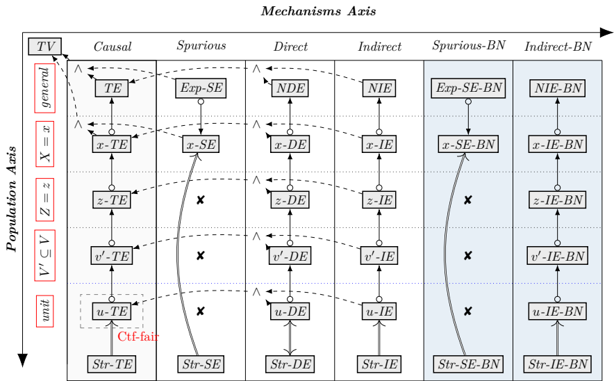
Figure 6.14: Fairness Map for the TV-family of measures. The horizontal axis represents the mechanisms (causal, spurious, direct, and indirect), and the vertical axis the events that capture increasingly more granular sub-populations, from general ( P(u) ) to unit-level. The bottom row contains structural measures. The arrow \Rightarrow indicates relations of admissibility, \circ \rightarrow of power, and \circ \dashrightarrow of decomposability.
