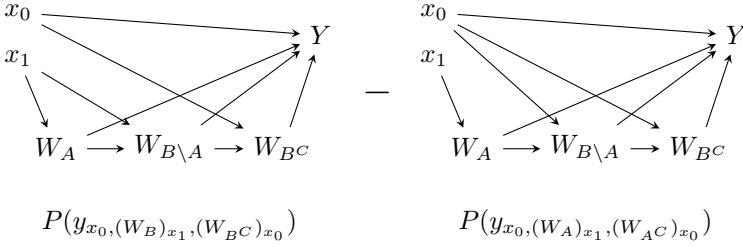
Figure 6.11: Quantity E\text{-IE}_{x_0, x_1}^{W_A, W_B}(y) as a graphical contrast.
