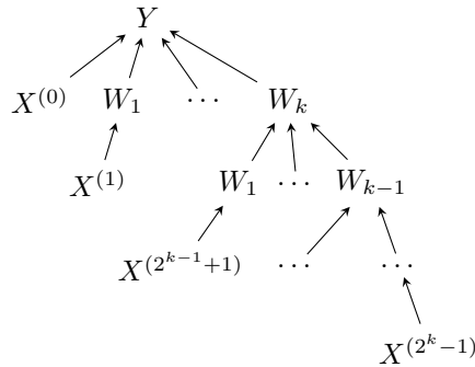
Figure 6.15: Visualization of how a path-specific potential response is obtained.
